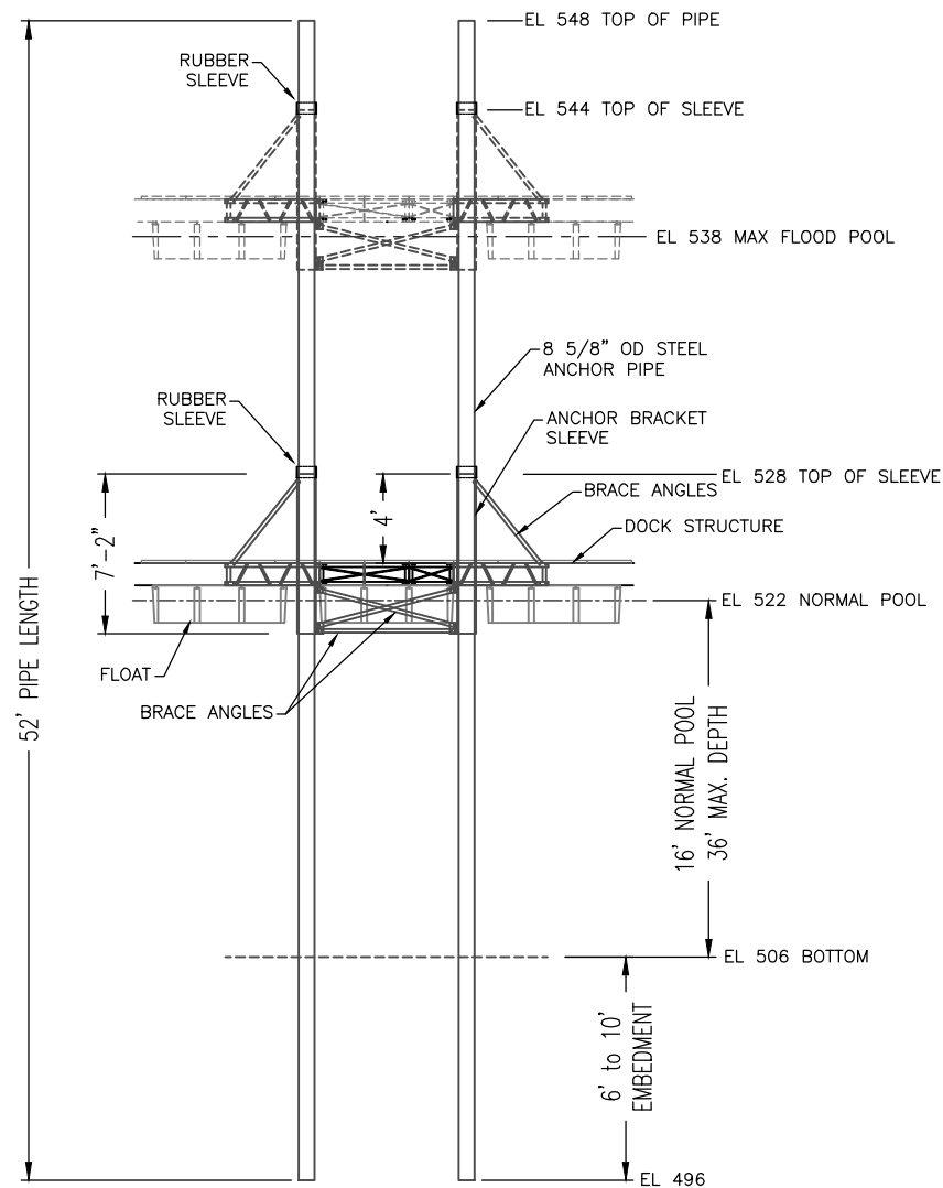
SECTION
