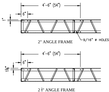
TYPICAL CORNERWALK HOLES
